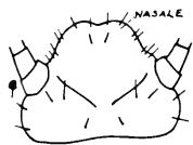
Fig. 196. Dorsal aspect of head.
